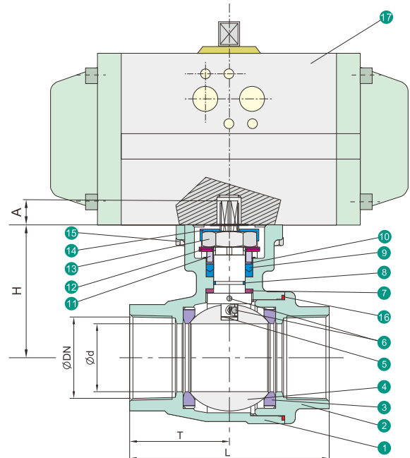
SIZE: 1/4" ~ 3"
